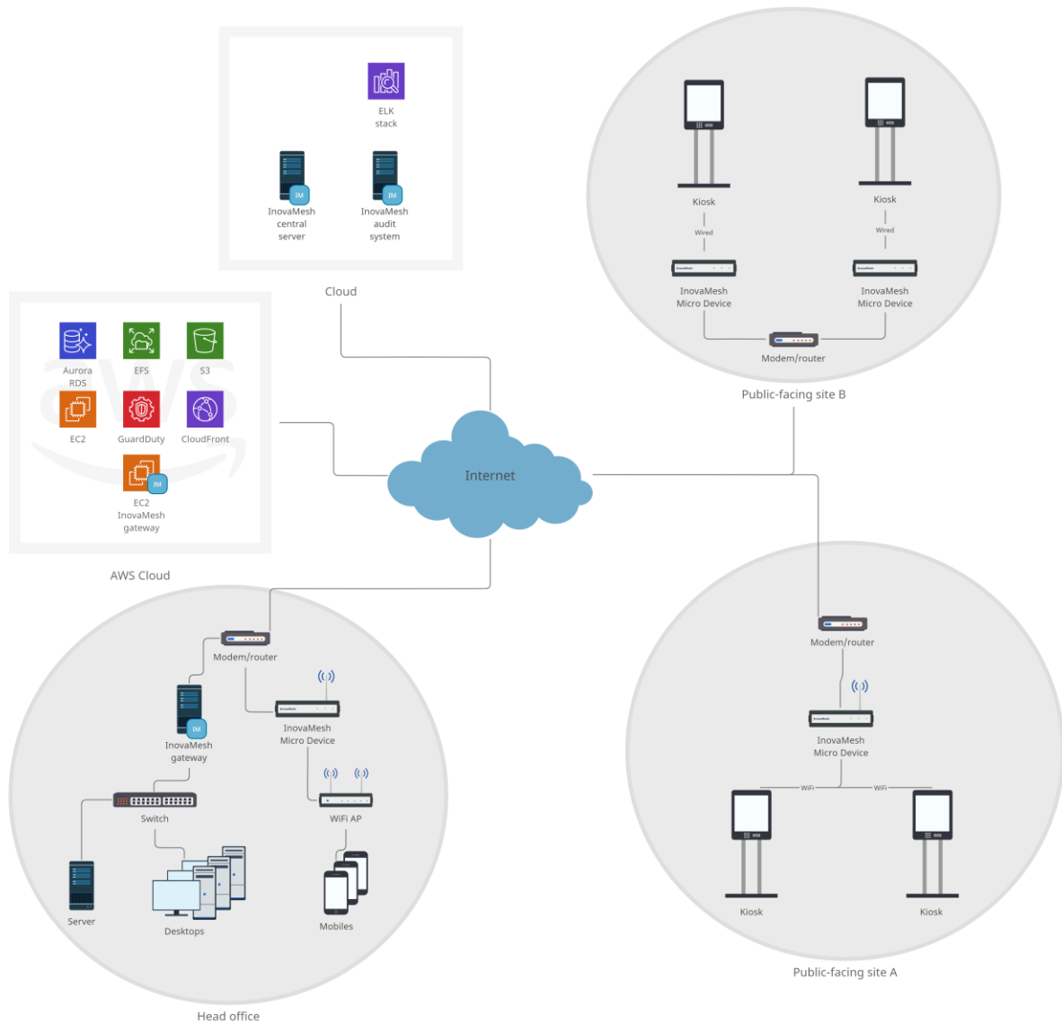
FIG 1. OVERALL NETWORK TOPOLOGY
